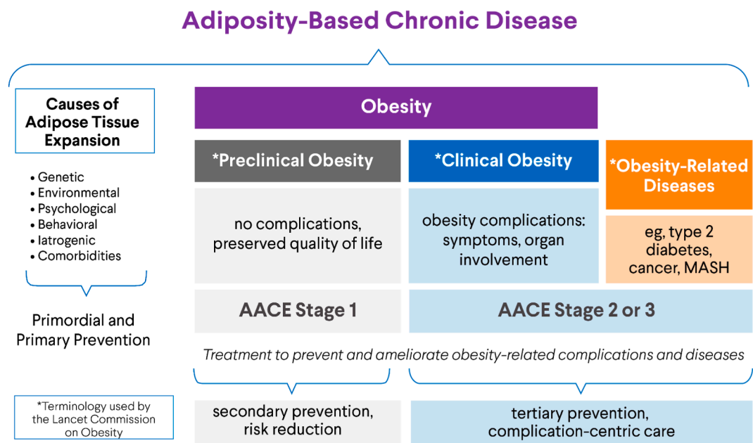
Fig. 1. Adiposity-based chronic disease and relationships involving the AACE obesity algorithm and terms used by the Lancet Commission on Obesity. MASH = metabolic dysfunction-associated steatohepatitis.
